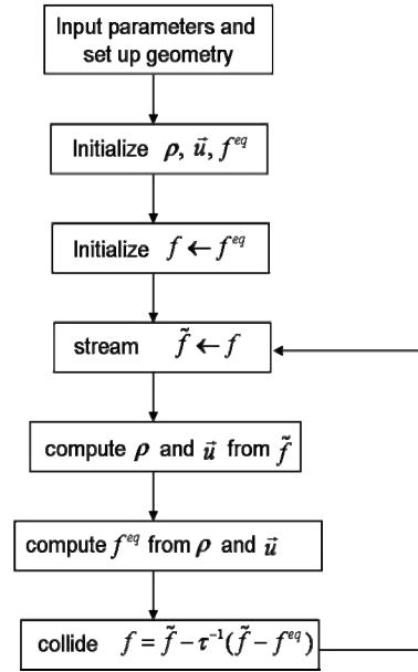
Fig. 3. Flowchart diagram.
